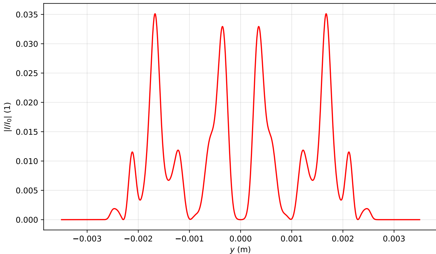
Intensity profile I(x=0, y, z=3.901)/I_0 , P_{in}=7.0P_{cr} , artificial time
